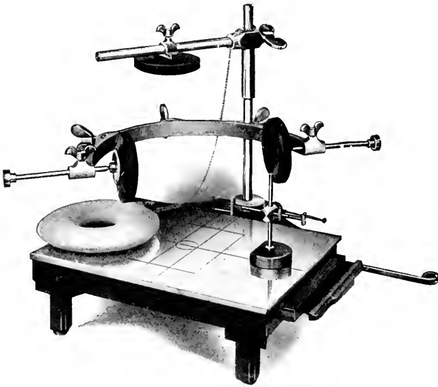
FIG. 104.—Sweet localiser.
